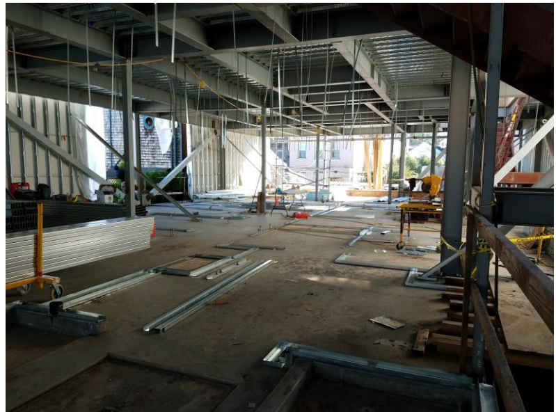
Interior Metal Stud Framing at 2nd Floor (February 7, 2018)
